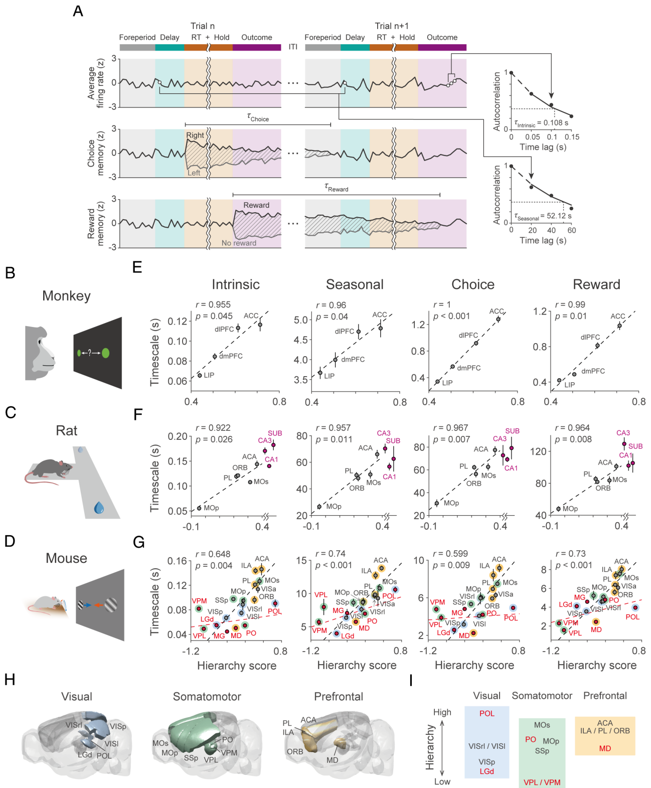
Fig. 1. Multiple timescales in the neocortex follow the same hierarchical gradient. (A) Estimation of multiple timescales using an autoregressive model is illustrated with hypothetical neural data. Intrinsic and seasonal timescales estimate the rate of change in correlated neural activity within and across trials, respectively, whereas choice- and reward-memory timescales quantify the decay of neural signals related to the animal's choice and its outcome, respectively. (B–D) Behavioral task for each species. Matching pennies task for monkeys (B), dynamic foraging task for rats (C), and visual discrimination task for mice (D). (E–G) Correlation between the timescales of neural activity and anatomical hierarchy score in monkeys (E), rats (F), and mice (G). Each dot and error bar, respectively, indicate the median and SE of the timescale within each area. In (F), black and pink dots represent data from the neocortex and hippocampus, respectively. Note that the data from the hippocampus (CA3, CA1, and SUB) do not have a precise hierarchy score. In (G), black and red dots represent data from the neocortex and thalamus, respectively. Blue, green, and yellow shading indicate the regions in the visual, somatomotor, and prefrontal areas, respectively. Dashed lines denote linear regression. The Pearson correlation coefficients ( r ) and P values are shown for the data pooled from all areas in each species. (H) Cortical areas and thalamic nuclei in the visual (Left), somatomotor (Middle), and prefrontal (Right) regions are rendered as in ref. 41. (I) Anatomical hierarchy of the same areas within each region is shown.
